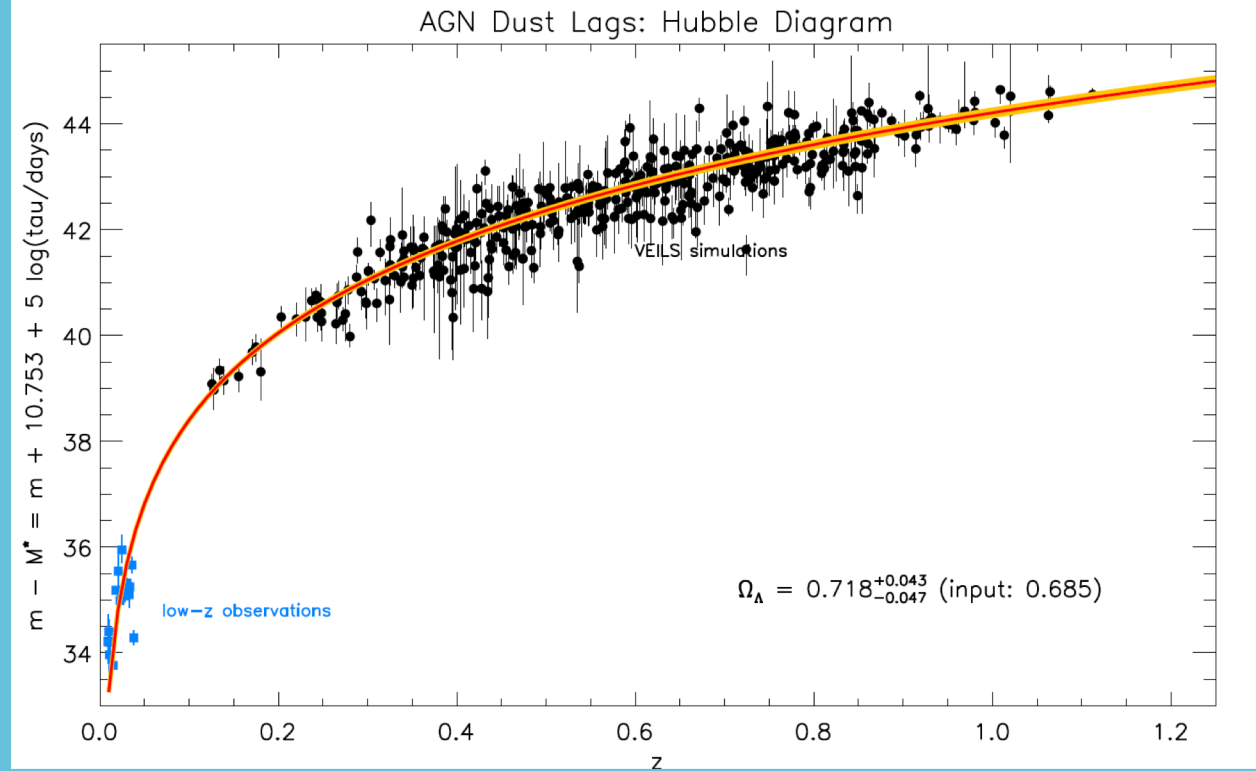
Towards creating a Hubble Diagram with AGN
