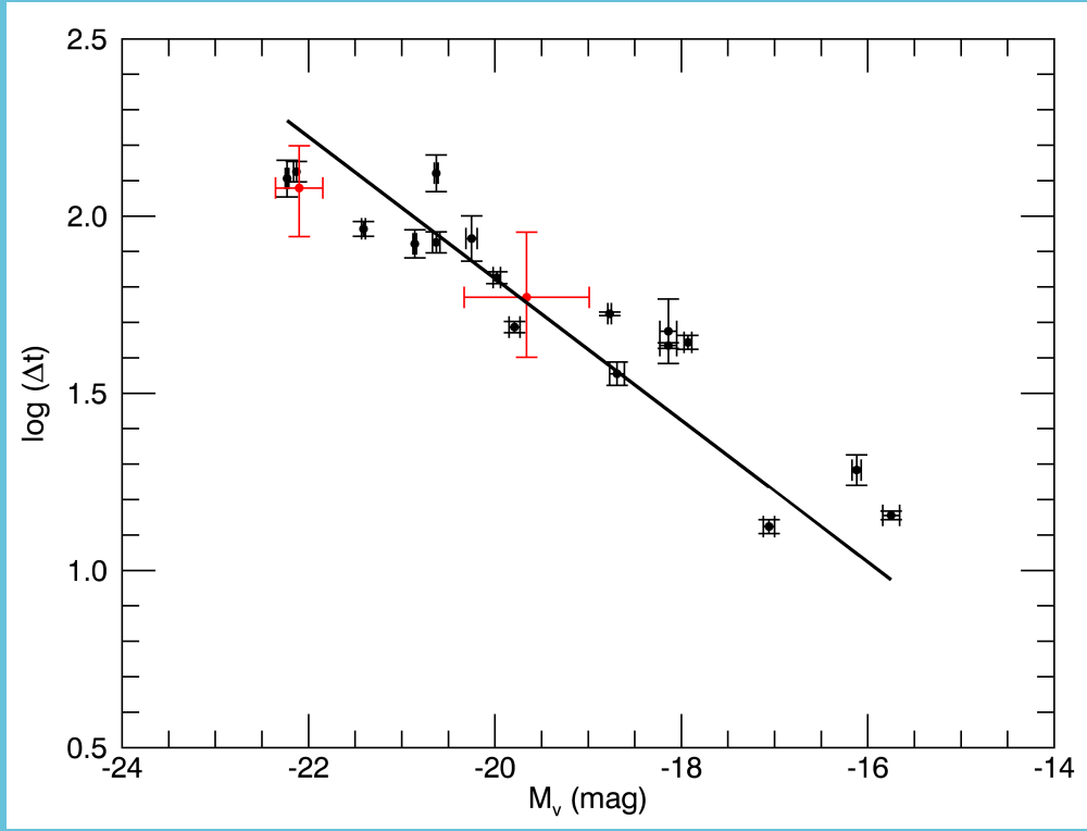
Further establishing the lag-luminosity relation
