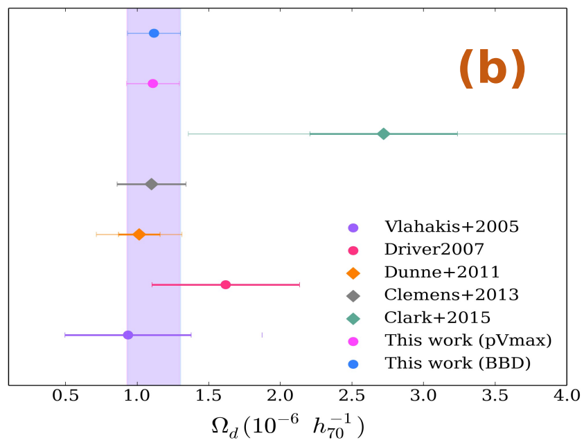
FIGURE 1 (Taken from Beeston et al., 2018) (a) Comparison of the observed DMF data and best-fitting SFs with the best-fitting SFs from the literature of observations of the DMF (b) Comparison of the cosmic dust density from this work to values the literature of observed DMFs (c) Comparison of the best-fitting SFs from this work to DMFs arising from semi-analytic models from P17 and cosmological hydrodynamic simulations from McK17 (d) Dust/stellar mass plane for observations from this work and literature with the binned values from P17
