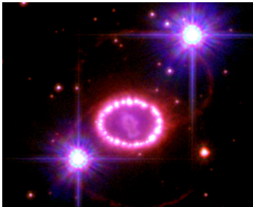
Neutrino Astrophysics & Particle Astrophysics
