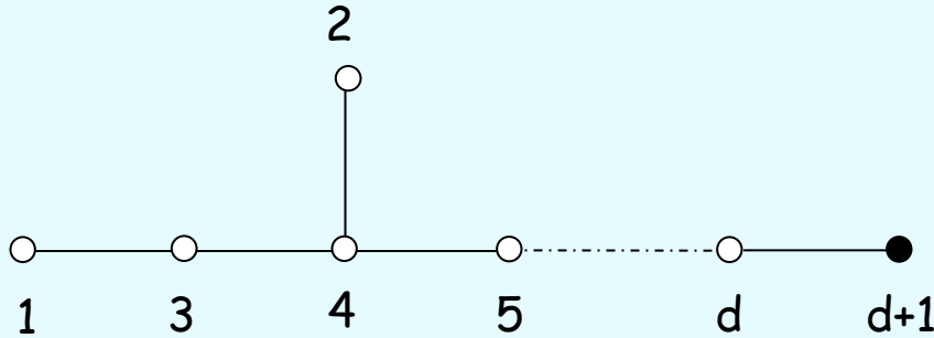
Dynkin diagram for E_{d+1}
